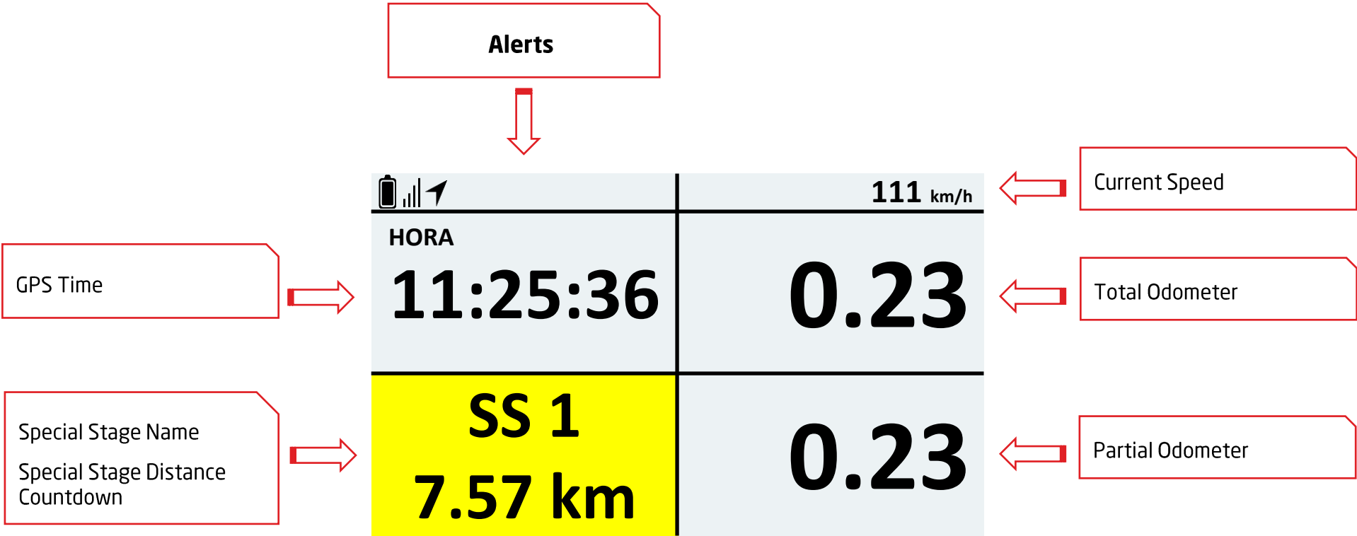
Image 1. MAIN SCREEN
